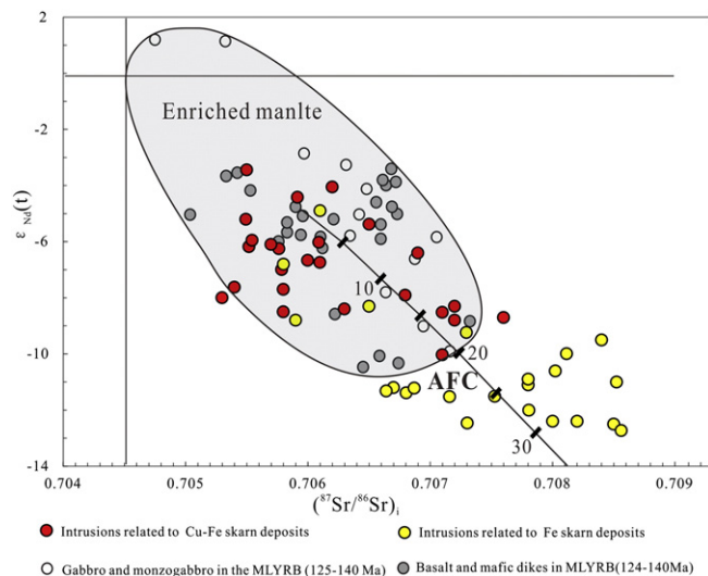
Fig. 7. Nd and Sr isotopic variation diagram for Late Mesozoic intrusions associated with the selected Cu–Fe and Fe skarn deposits in the Edong ore district, MLYRB. AFC: assimilation–fractional crystallization.
