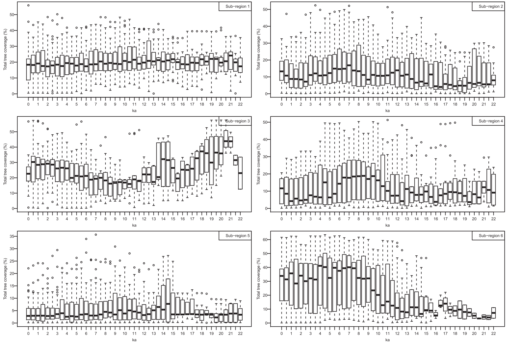
Fig. 5. Patterns of total tree cover in the six sub-regions over the last 22 kyr. Sub-region 1, south-eastern China; Sub-region 2, north-central China; Sub-region 3, north-eastern China and Russia Far East; Sub-region 4, eastern Tibetan Plateau; Sub-region 5, arid central Asia; and Sub-region 6, northern Mongolia and southern Siberia.
