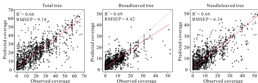
Fig. 2. Comparison of the AVHRR-derived observations of total tree, broadleaved, and needleleaved cover to the analogue-based percent cover estimates for modern pollen sites. R^2 is the coefficient of determination between observed and predicted tree cover and RMSEP is the root mean square error of prediction produced by the “leave-one-out” cross-validation.
