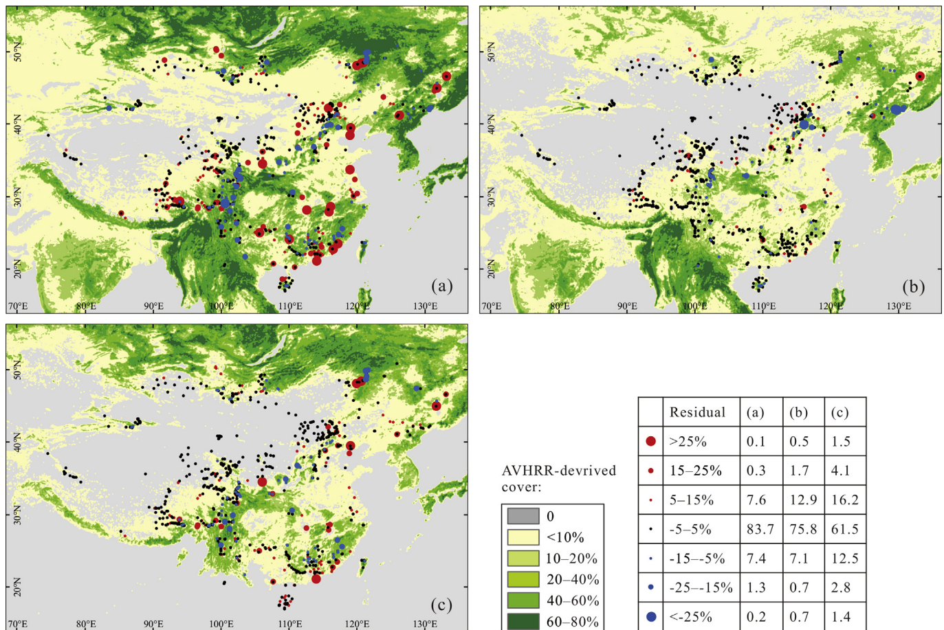
Fig. 3. The residuals between pollen-based reconstructions and AVHRR-derived observations for all the modern pollen sites: (a) total tree cover (the total tree cover for grids with values lower than 10% are set to 1% in the background map, but for all analyses we calculated them as the sum of broadleaved and needleleaved cover), (b) broadleaved cover, (c) needleleaved cover. The numbers in the table in the lower right of the figure show the proportion of modern pollen sites available within different ranges of residuals between pollen-based reconstructions and AVHRR-derived observations (reconstruction minus observation).
