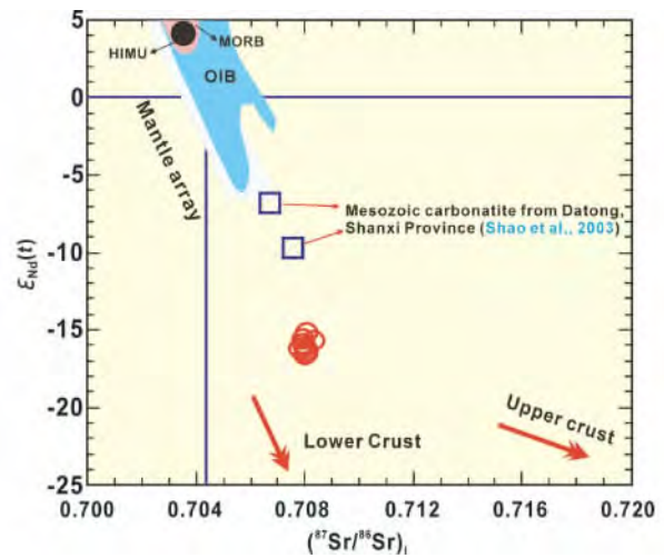
Fig. 5 Variations in initial ^{87}\text{Sr}/^{86}\text{Sr} ratios vs. \varepsilon_{\text{Nd}}(t) values for the carbonatite dykes of the northern NCC , China
