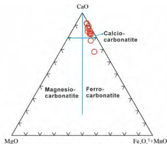
Fig. 3 Plot of the studied carbonatites on the CaO-MgO-( \text{Fe}_2\text{O}_3^{\text{T}} + \text{MnO} ) classification diagram (after Woolley and Kempe, 1989)
