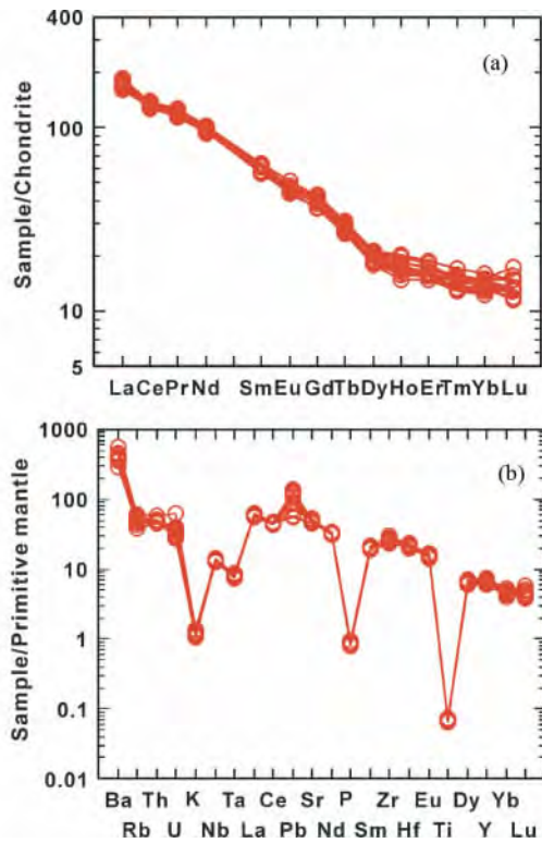
Fig. 4 Chondrite-normalized REE diagram ( a , normalization values after Anders and Grevesse , 1989) and primitive-mantle-normalized incompatible element distribution diagram ( b , normalization values after Sun and McDonough , 1989) for the carbonatite dykes of the northern NCC , China
