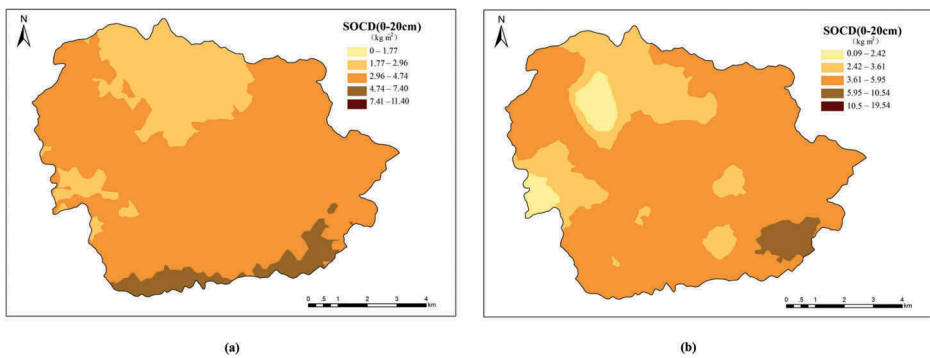
Figure 2. Temporal and spatial distribution of SOCD in the Houzhai basin (a. the SOCD spatial distribution in 1980; b. the SOCD spatial distribution in 2015).
