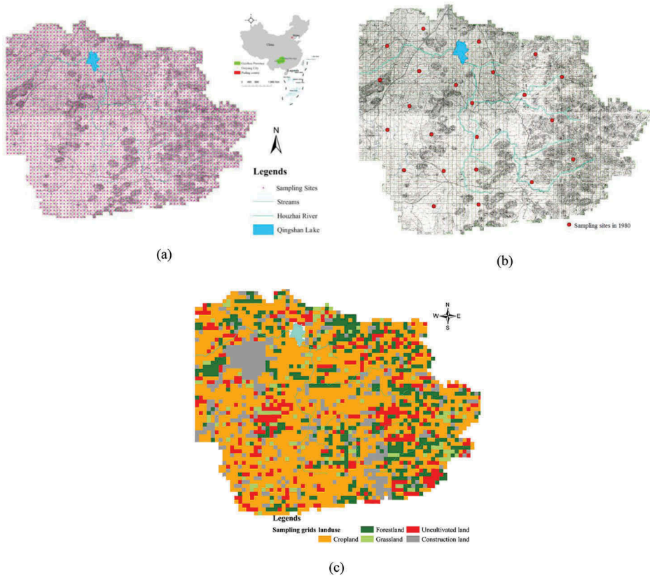
Figure 1. The distribution of sample sites in 2015 (a), in 1980 (b) and land use (c) in the Houzhai Basin.
