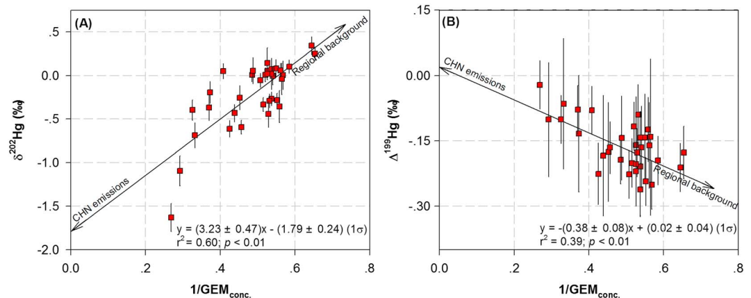
Figure 4. (a) \delta^{202}\text{Hg} versus 1/\text{GEM}_{\text{conc.}} and (b) \Delta^{199}\text{Hg} versus 1/\text{GEM}_{\text{conc.}} diagrams suggesting a binary mixing of regional background atmospheric GEM pool and Chinese (CHN) emissions of GEM.
