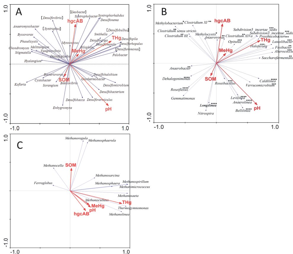
Fig. 6 Detrended correspondence analyses for the three primary Hg-methylating clades of (A) Deltaproteobacteria , (B) Firmicutes and (C) Archaea using 16S rRNA gene data.
