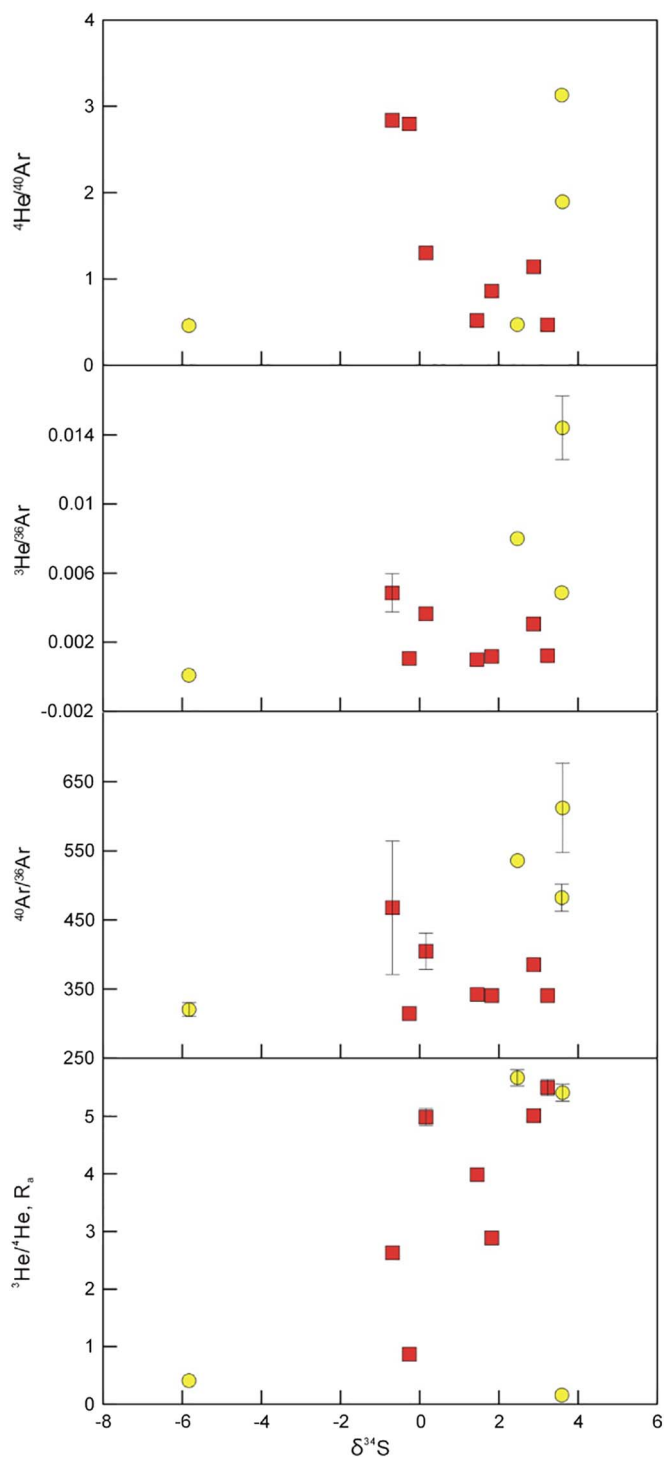
Fig. 5. {}^3\text{He}/{}^4\text{He} vs. \delta^{34}\text{S} , {}^{40}\text{Ar}/{}^{36}\text{Ar} vs. \delta^{34}\text{S} , {}^3\text{He}/{}^{36}\text{Ar} vs. \delta^{34}\text{S} , and {}^4\text{He}/{}^{40}\text{Ar} vs. \delta^{34}\text{S} for sulfides from the Zijinshan high sulfidation Cu-Au deposit and Wuziqilong Cu deposit. There is a poor relationship between S and He-Ar isotopes, though the decrease of \delta^{34}\text{S} with low {}^3\text{He}/{}^4\text{He} , {}^{40}\text{Ar}/{}^{36}\text{Ar} , {}^3\text{He}/{}^{36}\text{Ar} and high {}^4\text{He}/{}^{40}\text{Ar} ratios. Symbols as for Fig. 2.
