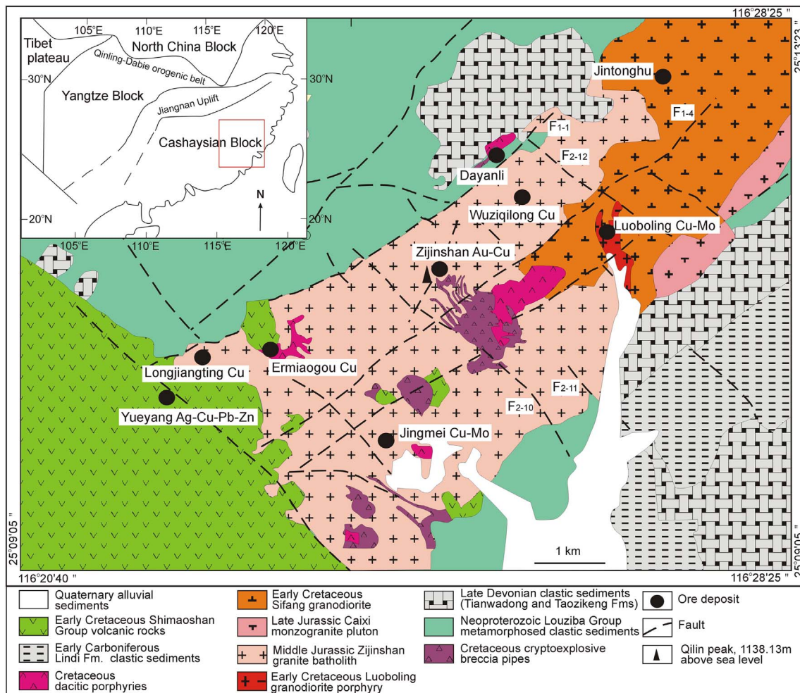
Fig. 1. Geological map of the Zijinshan orefield, South China modified from Hu and Zhou (2012) and Zhong et al. (2014).
