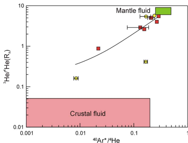
Fig. 2. ^{40}\text{Ar}^*/^4\text{He} vs. ^3\text{He}/^4\text{He} ( R_a ) of sulfides from the Zijinshan high sulfidation Cu-Au deposit and Wuziqilong Cu deposit. Symbols: red filled squares: Wuziqilong transitional Cu deposit; yellow filled circles: Zijinshan HS Cu-Au deposit. The linear correlation is obtained by least squares regression: ^3\text{He}/^4\text{He} ( R_a ) = 21.0 \times ^{40}\text{Ar}^*/^4\text{He} + 0.07 , r^2 = 0.69 . Error bars not displayed are concealed in the sample symbols, as follows. (For interpretation of the references to colour in this figure legend, the reader is referred to the web version of this article.)
