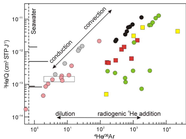
Fig. 4. {}^3\text{He}/\text{Q} vs. {}^4\text{He}/{}^{36}\text{Ar} for sulfides from the Zijinshan high sulfidation Cu-Au deposit and Wuziqilong Cu deposit. Symbols: red filled squares = Wuziqilong deposit; yellow filled squares = Zijinshan deposit; filled circles = Panasqueira arsenopyrite (Burnard and Polya, 2004); green filled circles = Ailaoshan Au deposit (Burnard et al., 1998); gray filled circle = East Pacific Rise sulfides (Turner and Stuart, 1992); pink filled circles = Iceland hydrothermal fluids (Poreda and Amorsson, 1992); solid horizontal lines = range in {}^4\text{He}/{}^{36}\text{Ar} of EPR vent fluids and plumes (Lupton et al., 1989; Lupton et al., 1995); box = Lucky Strike vent fluids (Jean-Baptiste et al., 1998). (For interpretation of the references to colour in this figure legend, the reader is referred to the web version of this article.)
