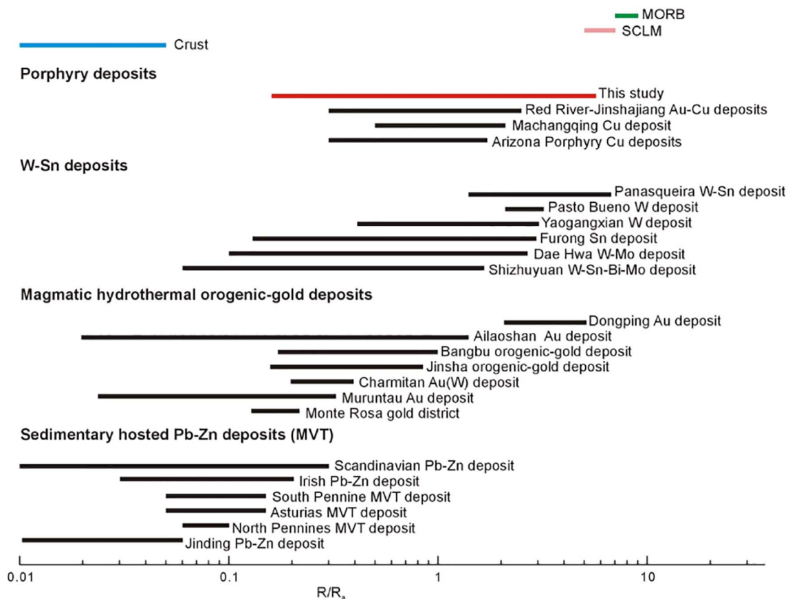
Fig. 6. ^3\text{He}/^4\text{He} of different types of ore deposits (data from Burnard et al., 1999; Burnard and Polya, 2004; Davidheiser-Kroll et al., 2014; Gautheron and Moreira, 2002; Graupner et al., 2006, 2010; Hu et al., 1998a, 1998b, 2004, 2012; Kendrick et al., 2001, 2002, 2005; Li et al., 2007, 2010; Mao and Li, 2003; Morelli et al., 2007; Pettke et al., 1997; Simmons et al., 1987; Stuart and Turner, 1992; Stuart et al., 1995; Sánchez et al., 2010; Tang et al., 2017; Wei et al., 2010; Wu et al., 2011). Most porphyry deposits have ^3\text{He}/^4\text{He} ratios lower than 2.5 R_a , while deposits from Zijinshan orefield have ^3\text{He}/^4\text{He} ratios up to 5.7 R_a . Most W-Sn deposits have ^3\text{He}/^4\text{He} ratios between 0.06 and 3.2 R_a , but there is an exception of Panasqueira W-Cu (Ag)-Sn deposit which has ^3\text{He}/^4\text{He} ratios up to 6.7 R_a . Most magmatic hydrothermal orogenic-gold deposits have ^3\text{He}/^4\text{He} ratios lower than 1.42 R_a , but with an exception of Dongping orogenic-gold deposit from Hebei Province, China, with ^3\text{He}/^4\text{He} ratios up to 5.2 R_a . Most sedimentary hosted Pb-Zn deposits (MVT) share ^3\text{He}/^4\text{He} ratios lower than 0.3 R_a . (For interpretation of the references to colour in this figure legend, the reader is referred to the web version of this article.)
