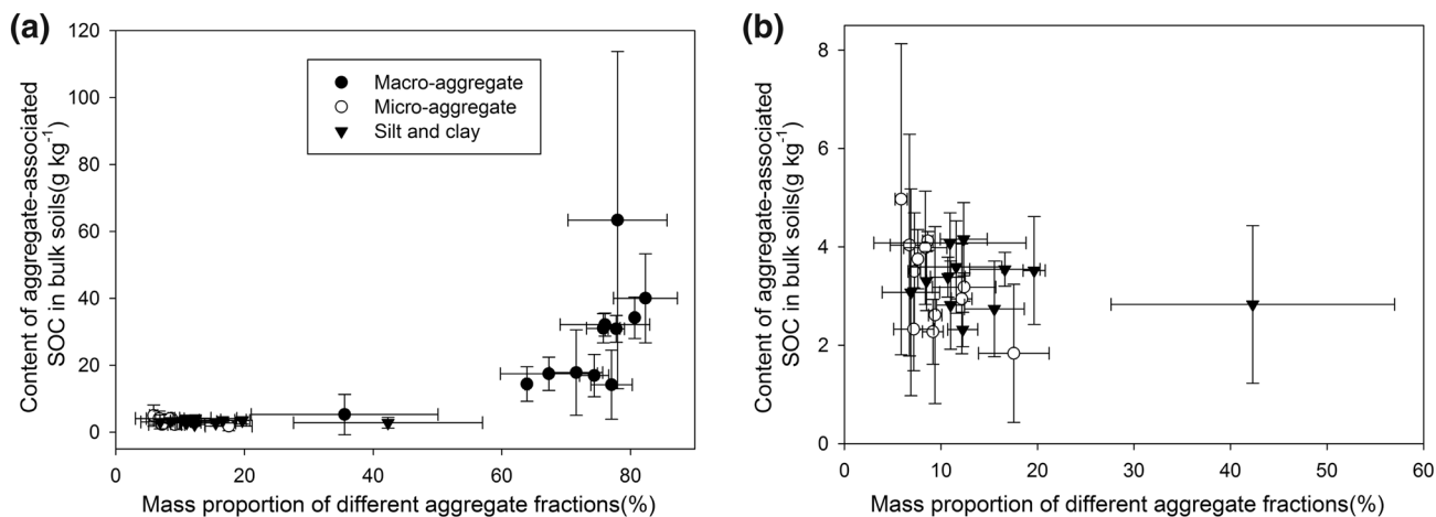
Fig. 3 Mass proportion of different aggregate fractions versus content of aggregate-associated SOC in bulk soils under different land uses. Error bars are SD of means (mean is an average from 0–10, 10–20, and 20–30 cm depth SOC content, n = 3 ). Plot a includes macro-aggregates, micro-aggregates, and silt and clay fractions. Plot b is a partially enlarged drawing of a , and includes micro-aggregates and silt and clay fractions only
