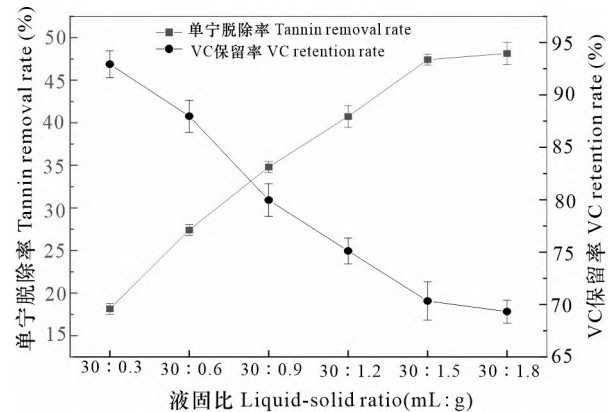
图 1 液固比对单宁脱除率和 VC 保留率的影响 Fig. 1 Effects of liquid-solid ratio on tannin removal rate and VC retention rate
