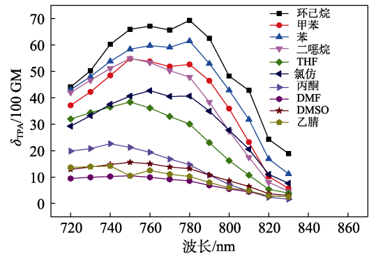
SP 溶液浓度为 10 μmol/L 图 8 SP 在各种溶剂中的双光子吸收截面与双光子激发波长的关系 Fig. 8 Two-photon absorption cross sections of SP in various solvents versus two-photon excited wavelengths
