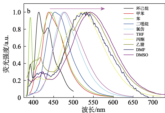
SP 溶液浓度为 1 \mu\text{mol/L} , \lambda_{\text{ex}}=360 \text{ nm}
