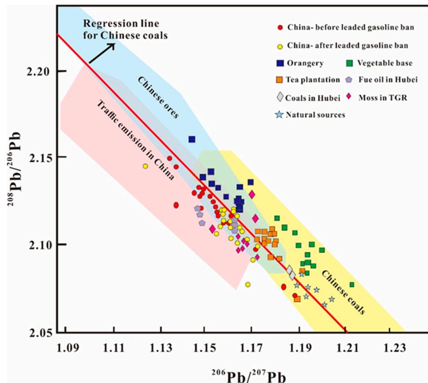
Figure 4. Lead isotope ratios ( 206 Pb/ 207 Pb vs. 208 Pb/ 207 Pb) in the soil samples. The regression line for Chinese coals was from Bi et al. (2017) [47]; unleaded gasoline and diesel exhausts and local coals (Hubei) from Bi et al. (2017) [47]; mosses from TGR from Liu et al. (2018) [18]; natural backgrounds were from [45,46,48,49].
