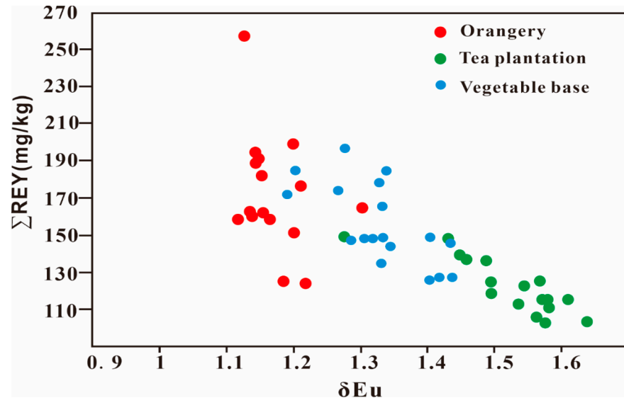
Figure 3. The δEu – ΣREY plot of three types of soils of farmland.
