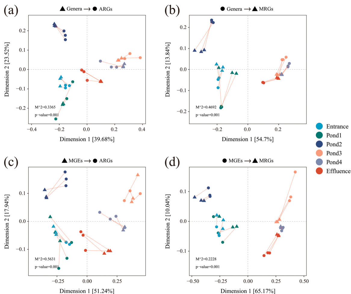
Fig. 4. Procrustes analysis with Spearman correlations displaying significant correlations between (a) genera and antibiotic resistance genes (ARGs), (b) genera and heavy metal(loid) resistance genes (MRGs), (c) mobile gene elements (MGEs) and ARGs, and (d) MGEs and MRGs. In the passive treatment of coal source acid mine drainage, the six sample sites were at the entrance of the first pond and the effluences of five ponds, named as Entrance, Pond1, Pond2, Pond3, Pond4, and Effluence, respectively.
