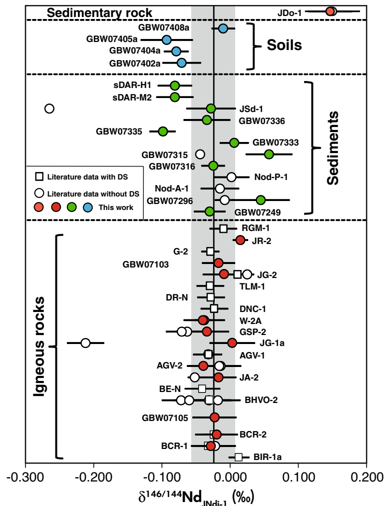
Figure 1. Comparison of \delta^{146/144}\text{Nd} values measured in this study with those reported in literature data. Vertical grey area represents \delta^{146/144}\text{Nd} value of BSE, which is -0.024 \pm 0.031\text{‰} ( 2s , n = 80 ) taken from McCoy-West et al. (2021). Filled brown, red, green, and blue circles represent stable Nd isotopic compositions measured in this study, while the open circles and squares represent the literature data with double spike (DS) and without double spike, respectively, summarised in Table 1. Range bars represent two standard deviations ( 2s ).
