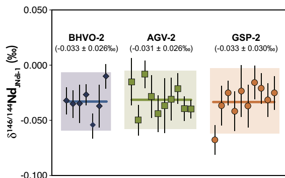
Figure 3. Intermediate measurement precision of the USGS geological reference materials BHVO-2, AGV-2 and GSP-2 after replicated digestion and processing through chemistry and being analysed separately. The complete dataset is shown in Table 2. Precision of \delta^{146/144}\text{Nd} values analysed here is better than \pm 0.030\text{‰} .
