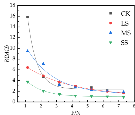
Figure 6. The change of B. striata leaf R with clamping force F .
