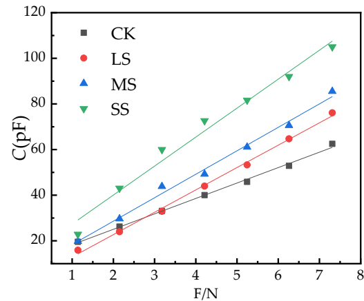
Figure 5. Variation of C of B. striata leaf with clamping force F .
