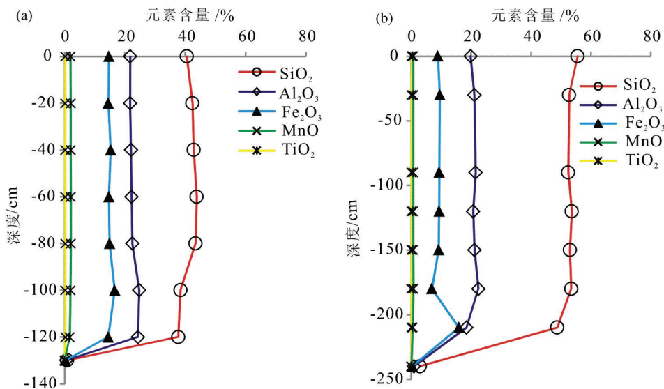
图3 难溶性元素在白云岩和石灰岩风化剖面中的地球化学特征 Fig.3 Geochemical characteristics of insoluble elements in the weathering profiles of dolomite and limestone
