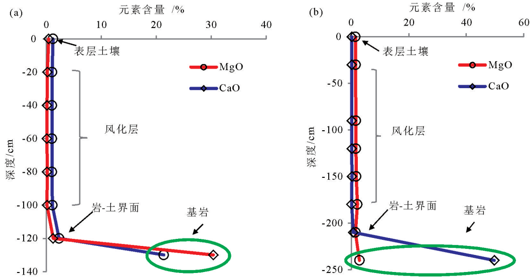
图2 CaO和MgO在白云岩和石灰岩风化剖面地球化学特征 a—白云岩;b—石灰岩 Fig.2 Characteristics of CaO and MgO in dolomite and limestone profiles a—Dolomite sonte; b—Limestone
