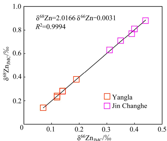
图7 羊拉铜矿床闪锌矿 Zn 同位素分馏图 Fig. 7 Diagram of Zn isotope fractionation in sphalerite, Yangla copper deposit
