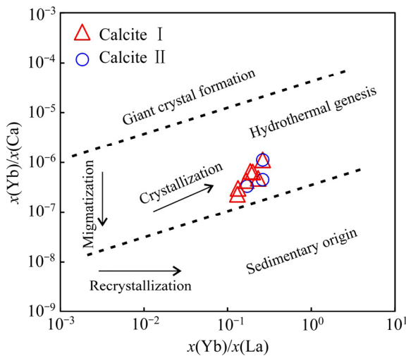
图 11 羊拉铜矿床铅锌矿石中方解石 x(\text{Yb})/x(\text{La}) — x(\text{Yb})/x(\text{Ca}) 图(底图据文献[69])
