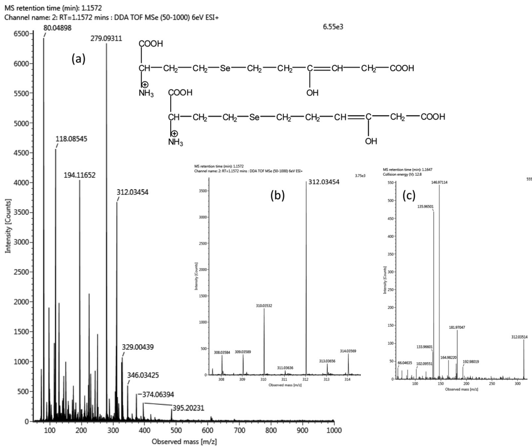
Fig. 6 Full scan spectrum (a), zoomed full scan spectrum (b), and MS/MS spectrum of the less hydrophobic isomer (c) of the selenohomocysteine-derived compounds with the experimental m/z 312.03454 ( ^{80}\text{Se} ), presented with putative structures in the inset. MS/MS spectrum of the more hydrophobic isomer couldn't be recorded because of low abundance.
