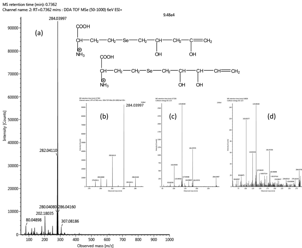
Fig. 5 Full scan spectrum (a), zoomed full scan spectrum (b), MS/MS spectrum of the more hydrophobic isomer (c) and MS/MS spectrum of the less hydrophobic isomer (d) of the selenohomocysteine-derived compounds with the experimental m/z 284.03997 ( ^{80}\text{Se} ), presented with putative structures in the inset.
