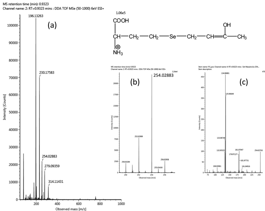
Fig. 3 Full scan spectrum (a), zoomed full scan spectrum (b) and MS/MS spectrum (c) of the selenohomocysteine-derived compound with the experimental m/z 254.02883 ( ^{80}\text{Se} ), presented with a putative structure in the inset.
