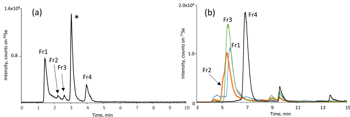
Fig. 1 (a) Strong cation exchange (SCX) – ICP-MS chromatogram of water soluble extract of C. violifolia , recorded on the ^{82}\text{Se} isotope. Fractions labelled #1–#4 were collected for further characterization on LC-Unispray-QTOFMS. “*” denotes to selenolanthionine. (b) Ion-pairing reversed phase (IP-RP) – ICP-MS chromatograms of the fractions #1–#4 collected from SCX – ICP-MS, recorded on the ^{77}\text{Se} isotope.
