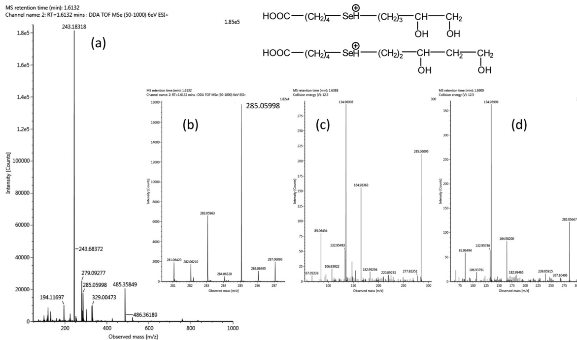
Fig. 8 Full scan spectrum (a), zoomed full scan spectrum (b), MS/MS spectrum of the less hydrophobic isomer (c) and MS/MS spectrum of the more hydrophobic isomer (d) of the compounds with the experimental m/z 285.05998 ( ^{80}\text{Se} ), presented with putative structures in the inset.
