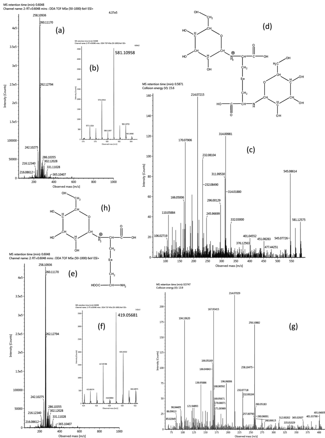
Fig. 9 Putative mono- and di- N -glycosides of selenolanthionine. Full scan spectrum (a), zoomed full scan spectrum with the experimental m/z 581.10958 ( 80 Se) (b), MS/MS spectrum (c) and structure of selenolanthionine-di- N -glycoside (d). Full scan spectrum (e), zoomed full scan spectrum with the experimental m/z 419.05681 ( 80 Se) (f), MS/MS spectrum (g) and structure of selenolanthionine- N -glycoside (h). Additional MS/MS spectrum of selenolanthionine-di- N -glycoside can be found in the ESI † (Fig. S10).
