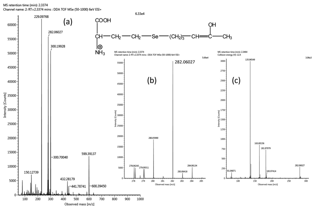
Fig. 4 Full scan spectrum (a), zoomed full scan spectrum (b) and MS/MS spectrum (c) of the selenohomocysteine-derived compound with the experimental m/z 282.06027 ( ^{80}\text{Se} ), presented with a putative structure in the inset.
