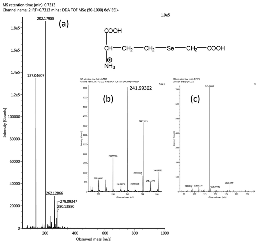
Fig. 2 Full scan spectrum (a), zoomed full scan spectrum (b) and MS/MS spectrum (c) of the compound with the experimental m/z 241.99302 ( ^{80}Se ), presented and putatively identified as Se-carboxymethyl-selenohomocysteine in the inset.
