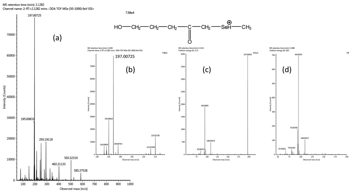
Fig. 7 Full scan spectrum (a), zoomed full scan spectrum (b), low fragmentation energy MS/MS spectrum (c) and high fragmentation energy MS/MS spectrum (d) of the compound with the experimental m/z 197.00725 ( ^{80}\text{Se} ), presented with a putative structure in the inset.
