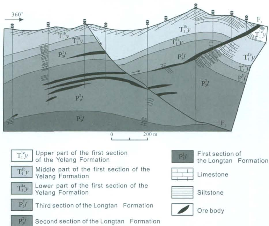
Figure 10 Map of the 32-32' exploration section of the Zimudang gold deposit (modified from Wang et al., 1994).
