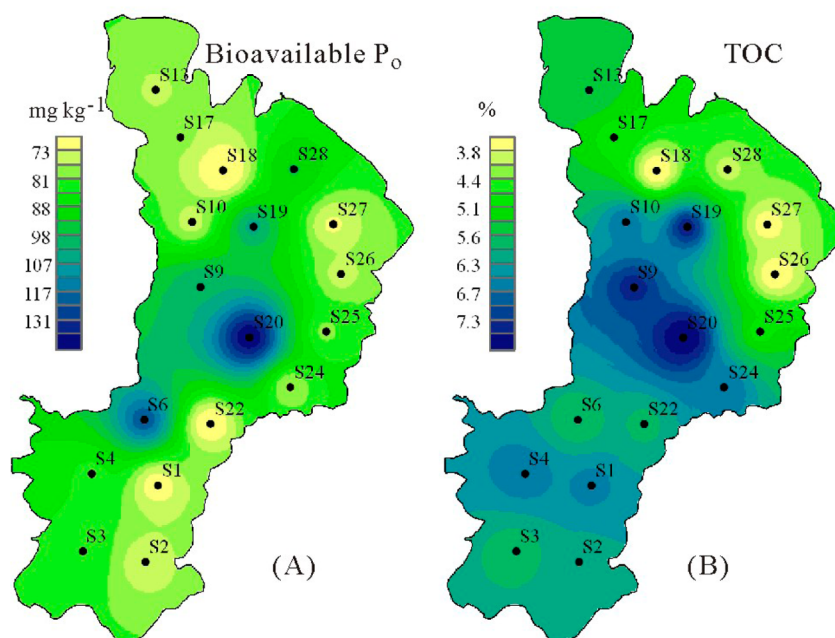
Figure 4. Spatial distributions of bioavailable P_o (A) and TOC (B) in surface sediments of Dianchi Lake. The sum of bioavailable P_o was calculated by P_o hydrolyzed in the H_2O , NaHCO_3 , and NaOH fractions by the combination of APase, PDEase, and phytase.
