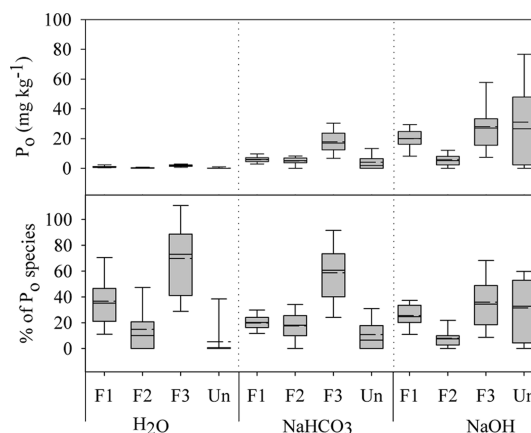
Figure 2. Contents and relative abundance of labile monoester P (F1), diester P (F2) and phytate-like P (F3), and unknown P o (Un) in the H 2 O, NaHCO 3 , and NaOH fractions, respectively. The lower boundary of each box indicates the 25th percentile, the full line within the box shows the median, the dashed line represents the mean, and the upper boundary shows the 75th percentile. Error bars indicate the 95th and 5th percentiles.
