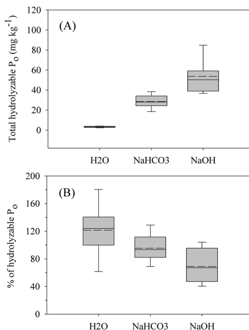
Figure 3. Summary of total hydrolyzable P o in H 2 O, NaHCO 3 , and NaOH fractions of sediments from Dianchi Lake: (A) the contents, (B) the percentage of P o released in according fractions. The lower boundary of each box indicates the 25th percentile, the full line within the box is the median, the dashed line shows the mean, and the upper boundary is the 75th percentile. Error bars indicate the 95th and 5th percentiles.
