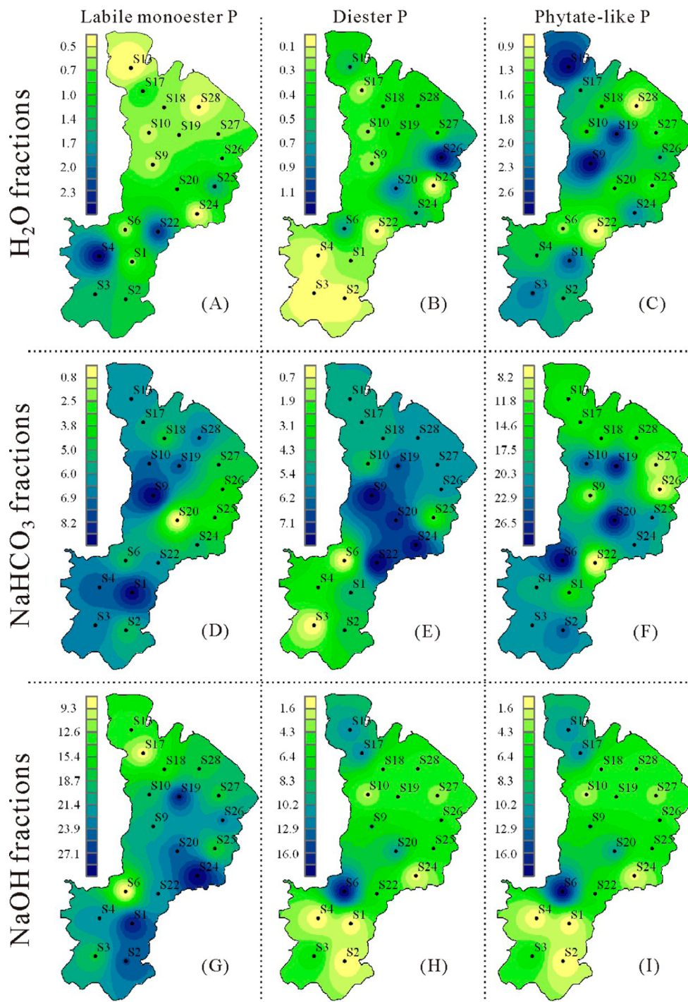
Figure 1. Spatial distribution of contents of P_o species ( \text{mg kg}^{-1} d.w.) characterized by phosphatase in the \text{H}_2\text{O} , \text{NaHCO}_3 , and \text{NaOH} fractions.
