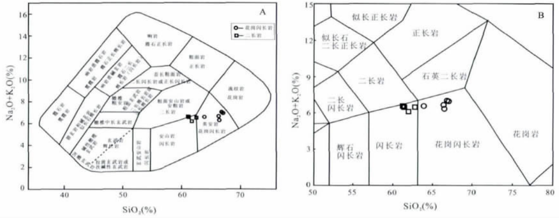
图 3 叶城县库喀阿孜铅-锌-(铜-钨)多金属矿区侵入岩的 \text{Na}_2\text{O}+\text{K}_2\text{O}-\text{SiO}_2 (TAS)图解(底图据文献[20,21]修改,图例同图 3A) Fig. 3 The \text{Na}_2\text{O}+\text{K}_2\text{O}-\text{SiO}_2 (TAS) diagram of the intrusive rocks from the Kukaazi Pb-Zn-(Cu-W) polymetallic deposit, Yecheng (modified from ref. [20,21], legends in Fig. 3A)
