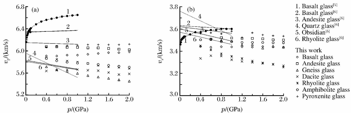
Fig. 2 v_p and v_s of glass under high pressure up to 2.0 GPa
