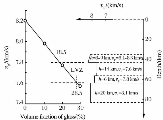
Fig. 5 Change of v_p of mantle rock with increasing content of glass in upper mantle (The profile of velocity versus depth is cited and modified from Ref. [25])
