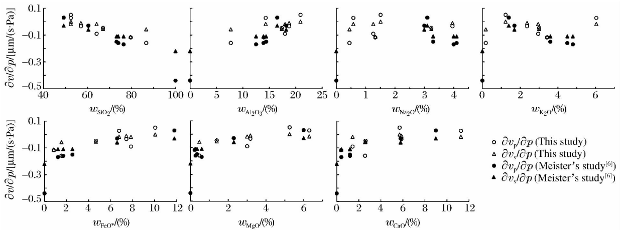
Fig. 3 Variations of pressure derivatives of v_p and v_s with chemical compositions in the glasses
