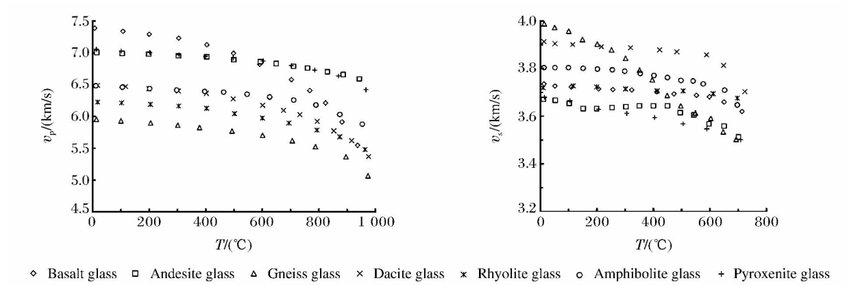
Fig. 4 Temperature effects on v_p and v_s of the glasses at 2.0 GPa
