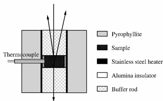
Fig. 1 Schematic representation of sample assembly
