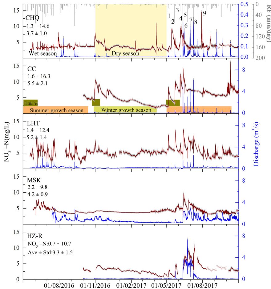
Fig. 2. The time series of in-situ [NO_3^- - N] and Q at the five sites. The shaded gray area associated with [NO_3^- - N] and Q represents the uncertainty of calibration. The light-yellow area represents the dry season (shown for CHQ but relevant for all sites). Gaps in the continuous record indicate missing data. To show the discharge clearly, wet season rainfall events have been numbered and the discharge scale at CHQ is smaller than other sites. Similarly, rainfall (RF), although measured at only LHT is only shown on the first time series. The abbreviations of Til and Fer in CC mean tillage and fertilization, respectively. The color shading in CC shows the time schedule of major agricultural activities across this KCZ. (For interpretation of the references to color in this figure legend, the reader is referred to the web version of this article.)
