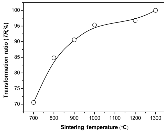
Fig. 2 The transformation ratio ( TR , %) of Zn into the \text{ZnCr}_2\text{O}_4 spinel structure after sintering the mixture of \text{ZnO} + \text{Cr}_2\text{O}_3
