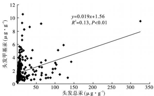
图 2 贵州汞矿区居民头发总汞和甲基汞含量之间的关系 Fig. 2 Correlation between hair T-Hg and MeHg concentrations for the residents from different Hg mining areas in Guizhou Province
