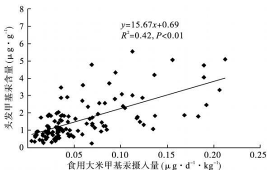
图 4 万山汞矿区居民食用大米甲基汞摄入量和头发甲基汞含量的关系 Fig. 4 Correlation between hair MeHg concentrations and MeHg intake from rice for the residents in Wanshan Hg mining area
