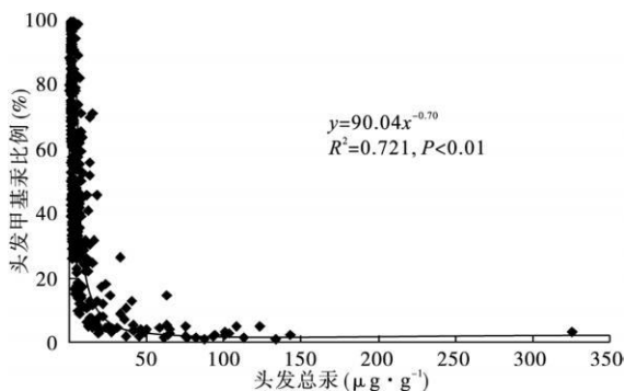
图 3 贵州汞矿区居民头发总汞和甲基汞比例含量之间的关系 Fig. 3 Correlation between T-Hg concentrations and MeHg percentages as Hg in the hair for the residents from different Hg mining areas in Guizhou Province
