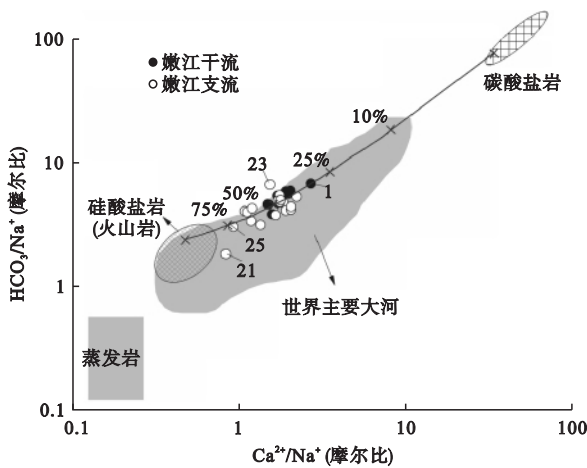
图8 Ca/Na和HCO 3 /Na的相互变化关系(端员值引自Gaillardet et al., 1999) Fig.8 Correlations between Ca/Na and HCO 3 /Na
