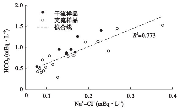
图7 (Na-Cl)和HCO 3 - 的相互变化关系(不包括23号样品) Fig.7 Correlations between (Na-Cl) and HCO 3 - (except for sample 23)
