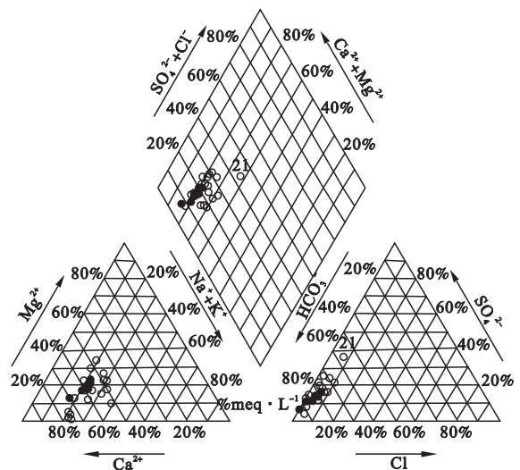
图 3 嫩江水系河水样品 Piper 图 Fig. 3 Piper diagram of the river water samples from Nenjiang Basin rivers
