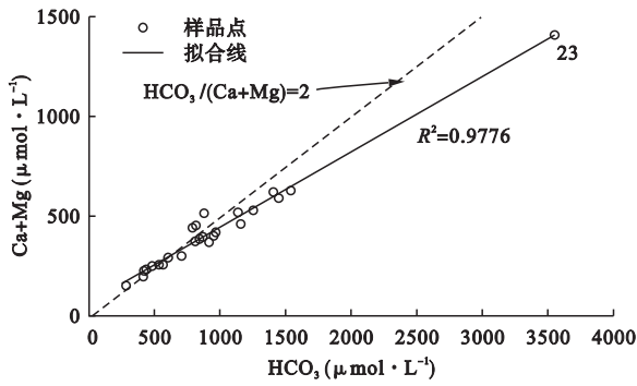
图6 HCO 3 - 和Ca 2+ +Mg 2+ 的相互关系 Fig.6 Correlations between HCO 3 - and Ca 2+ +Mg 2+
