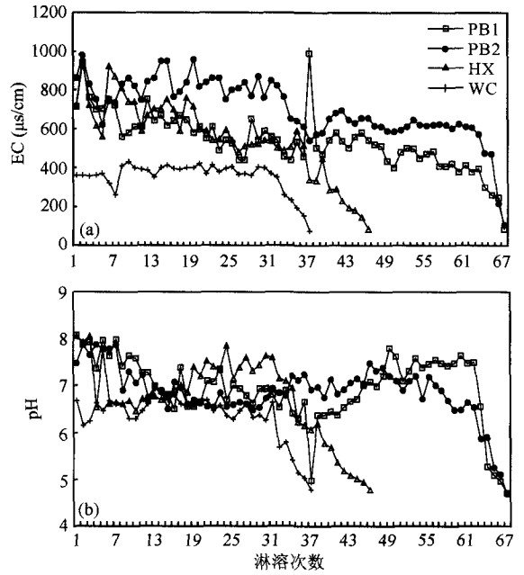
图3 随淋溶作用进程淋出液中 EC、pH 的变化 Fig. 3 The variation of EC and pH of leached solution along with leaching of carbonate rocks
