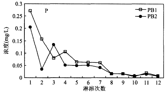
图 7 随淋溶作用进程淋出液中 P 的浓度变化 Fig. 7 The concentration variation of P of leached solution along with leaching of carbonate rocks
