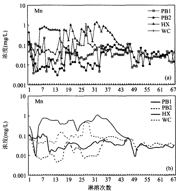
图 6 随淋溶作用进程淋出液中 Mn 的浓度变化 Fig. 6 The concentration variation of Mn of leached solution along with leaching of carbonate rocks
