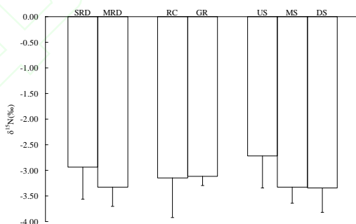
图3 不同环境条件下黄壤区地表凋落物 \delta^{15}\text{N} 均值 Fig.3 The mean \delta^{15}\text{N} value of litters in different environmental conditions in yellow soil areas
