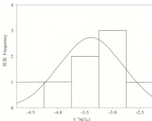
图2 黑色石灰土区地表凋落物 \delta^{15}\text{N} 值的频数分布直方图 Fig.2 Frequency histogram for \delta^{15}\text{N} values of litters in black calcareous soil areas
