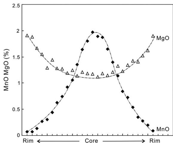
Fig. 6. The compositional profile of garnet.
