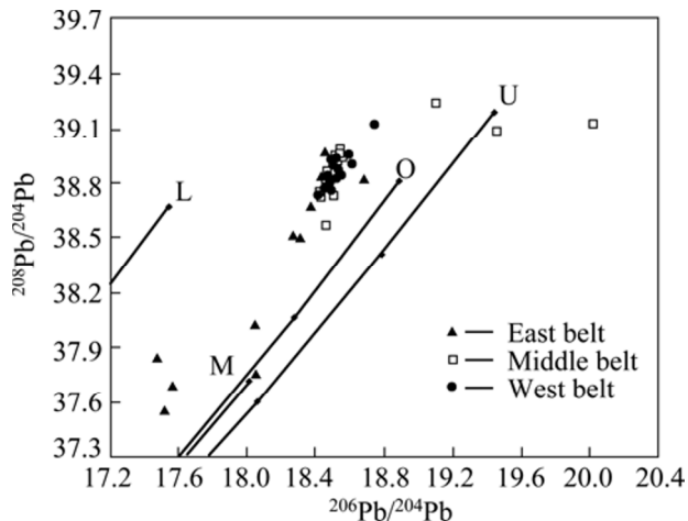
Fig. 7 ^{208}\text{Pb}/^{204}\text{Pb} vs ^{206}\text{Pb}/^{204}\text{Pb} growth curve of Dachang ore field: M—Upper mantle; L—Lower crust; O—Orogen; U—Upper crust [31]
