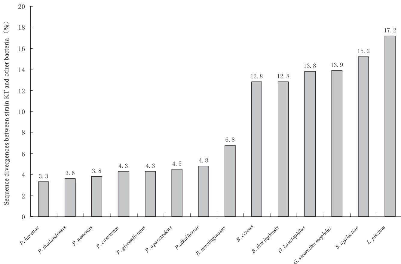
FIG. 1. The sequence divergence comparisons of the 16S rRNA genes between strain KT and other bacteria.
