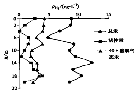
图 3 不同形态汞随水深的分布趋势 Fig.3 The trend of mercury species distribution in water column
