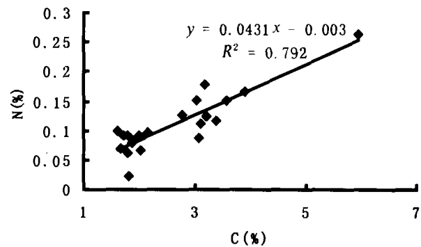
图 2 洱海沉积物中有机碳和氮的相关关系 Fig. 2 The relation between organic carbon and nitrogen in sediments of Erhai Lake
