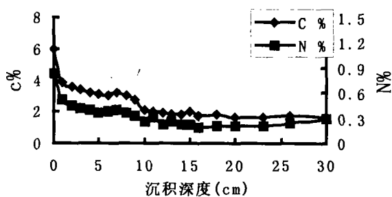
图 1 洱海沉积物中有机碳、氮垂直分布曲线 Fig. 1 The distribution of organic carbon and nitrogen in the sediments of Erhai Lake
